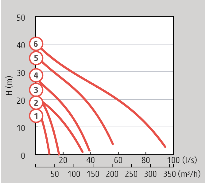
N versions – Minex – Matador – 50 Hz
