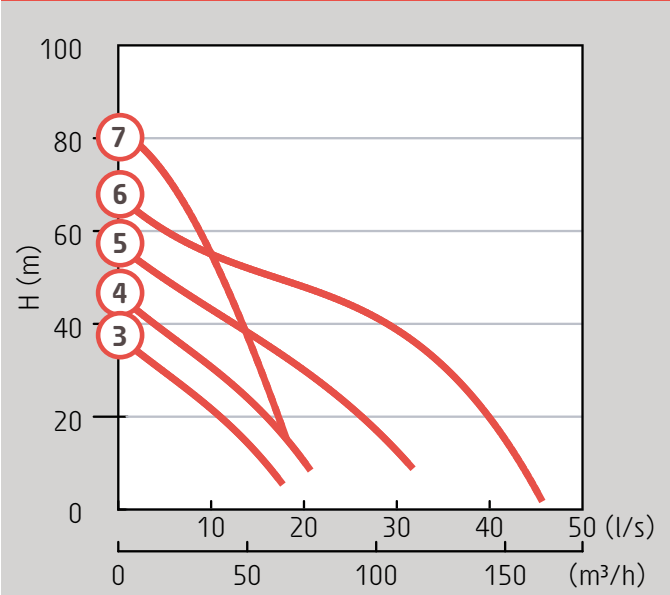
H versions – Minor – Matador – 50 Hz
