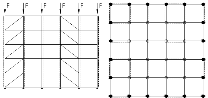
Y vertical brace position: - one brace per every third bay
