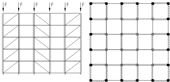
X vertical brace position: - one brace per every other bay
