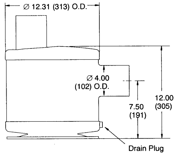
0541-1134 in (mm)
