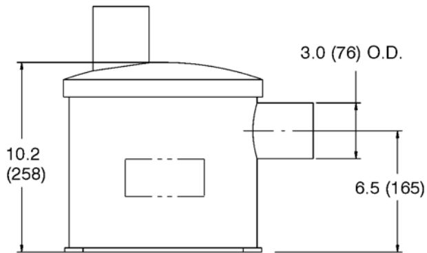
0541-1270 in (mm)
