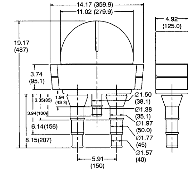
0155-3216 in (mm)
