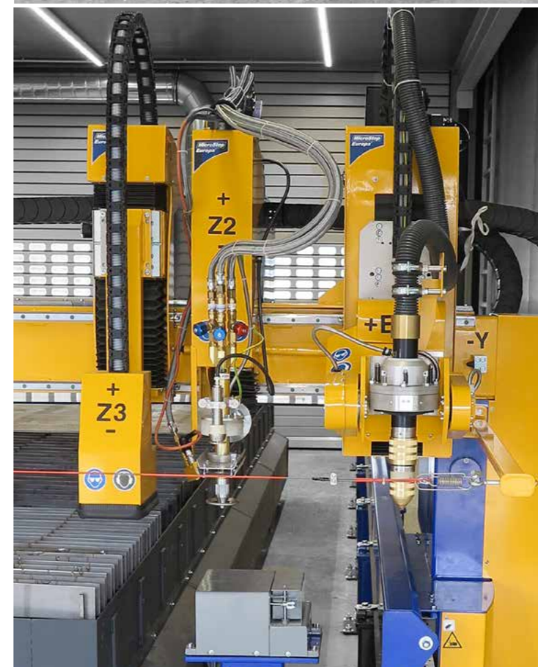
Configuration of MasterCut machine with a bevel head, an oxyfuel torch and a punch marker
